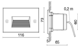
LUCE ASIMMETRICA ASYMMETRICAL LIGHT 24V
